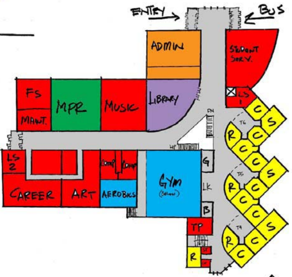
FLOOR PLAN - LEVEL 1 OPTION H 1"=40'
